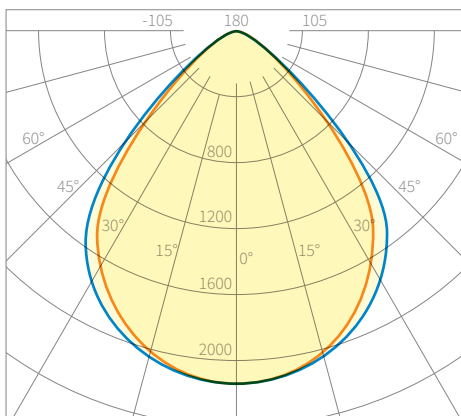
Measured* light distribution curve of temilux® ID
