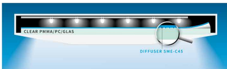
Diffuser SME-C45 with microstructures facing away from LEDs for homogen light
